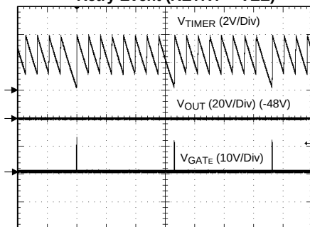
Retry Event ( \overline{\text{RETRY}} = V_{EE} )
