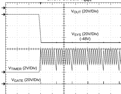
Short Circuit V_{\text{OUT}}
