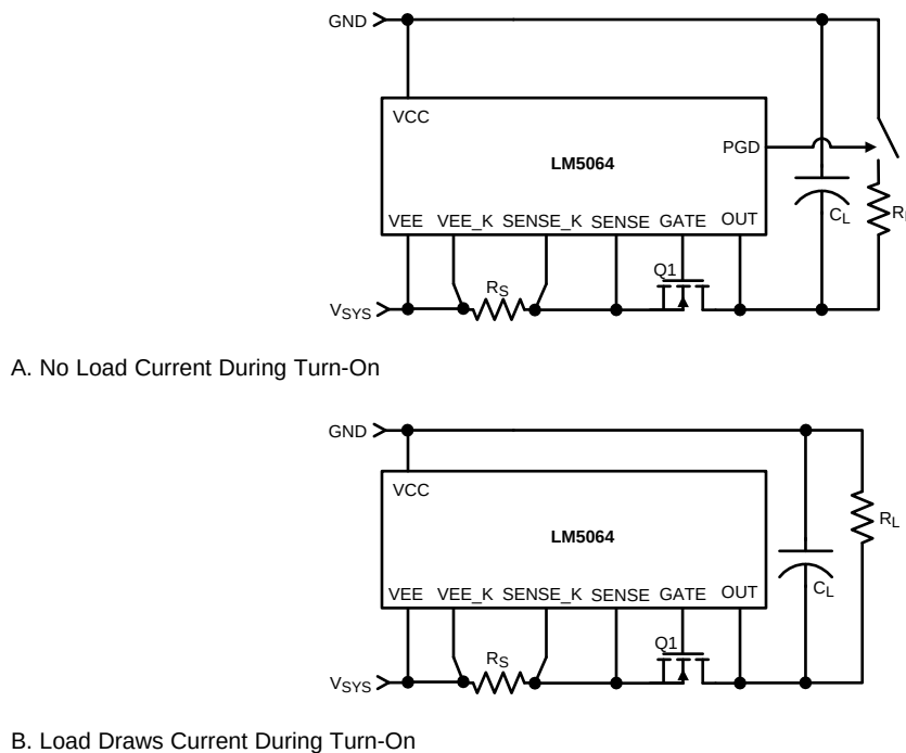
Figure 8. Current During Turn-On
