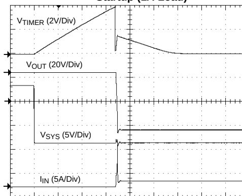
Startup (1A Load)
