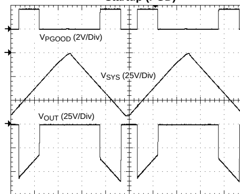
Startup (PGD)
