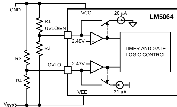
Figure 11. Programming the Four Thresholds
