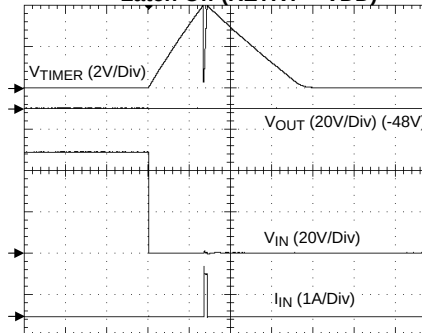
Latch Off ( \overline{\text{RETRY}} = V_{DD} )
