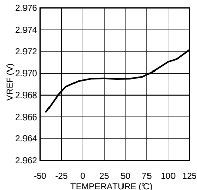
Reference Voltage
