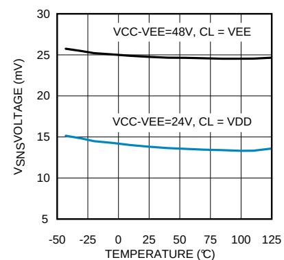
V_{\text{SNS}} (SENSE_K-VEE_K) at Power Limit Threshold R_{\text{PWR}} = 75\text{ k}\Omega
