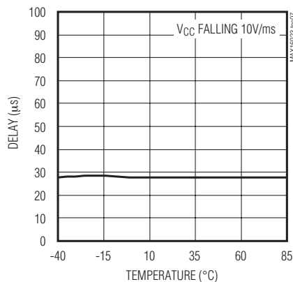
V_{CC} FALLING TO RESET DELAY vs. TEMPERATURE
