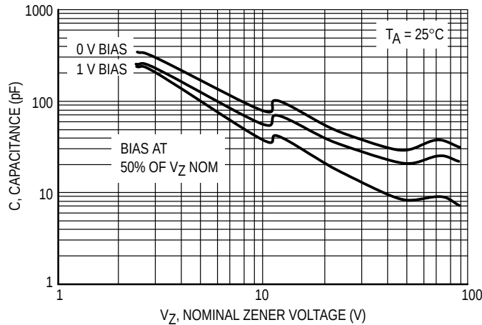
Figure 5. Typical Capacitance
