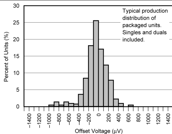
Figure 5-14. Offset Voltage Production Distribution V_S = \pm 5\text{V}
