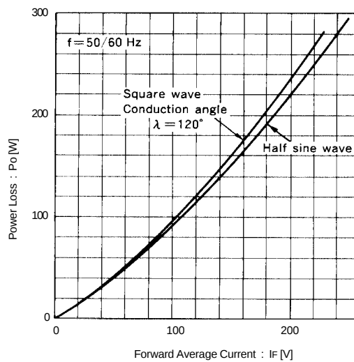
Forward Average Current vs. Power Loss
