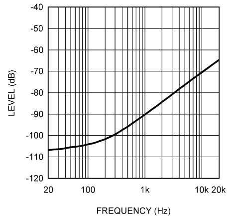
Crosstalk vs Frequency V_{DD} = \pm 75V
