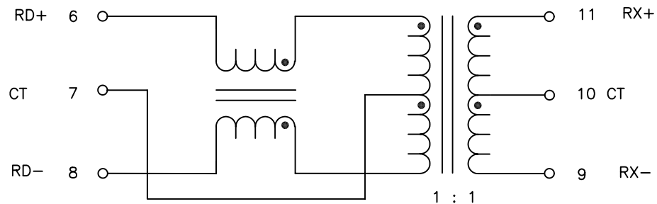
SCHEMATIC
