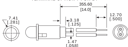
24 AWG WIRE LEADS - TERMINAL OPTION 3 FOR 6" WIRE LEAD TERMINAL OPTION 7 FOR 14"
