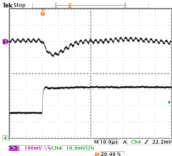
Fig-2.5V-6: Output voltage response for V_{out}=2.5V to positive load current step-change from 3A to 6A with slew rate of 5A/\mu s at V_{in}=5.0V . C_o=47\mu F \times 2 ceramic.
