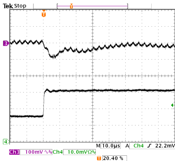
Fig-3.3V-6: Output voltage response for V_{out}=3.3V to positive load current step-change from 3A to 6A with slew rate of 5A/\mu s at V_{in}=5.0V . C_o=47\mu F \times 2 ceramic.
