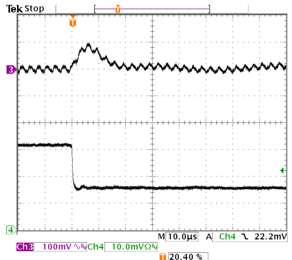
Fig-2.5V-7: Output voltage response for V_{out}=2.5V to positive load current step-change from 6A to 3A with slew rate of -5A/\mu s at V_{in}=5.0V . C_o=47\mu F \times 2 ceramic.
