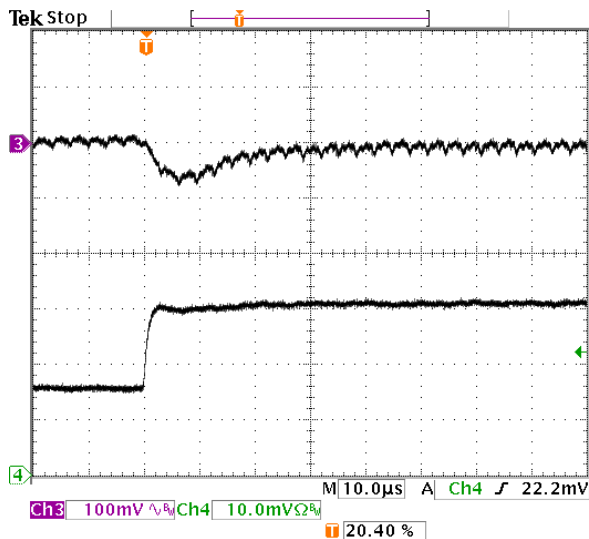
Fig-1.0V-6: Output voltage response for V_{out}=1.0V to positive load current step-change from 3A to 6A with slew rate of 5A/\mu s at V_{in}=5.0V . C_o=47\mu F \times 2 ceramic.
