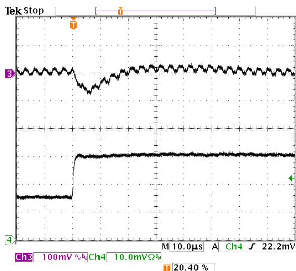
Fig-1.8V-6: Output voltage response for V_{out}=1.8V to positive load current step-change from 3A to 6A with slew rate of 5A/\mu s at V_{in}=5.0V . C_o=47\mu F \times 2 ceramic.
