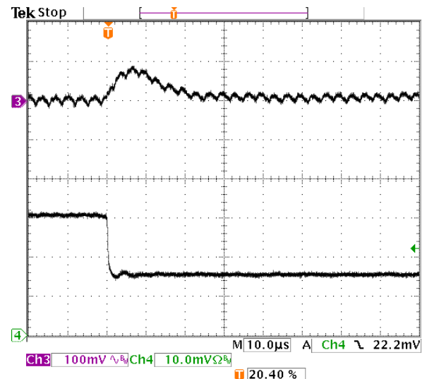
Fig-1.2V-7: Output voltage response for V_{out}=1.2V to positive load current step-change from 6A to 3A with slew rate of -5A/\mu s at V_{in}=5.0V . C_o=47\mu F \times 2 ceramic.
