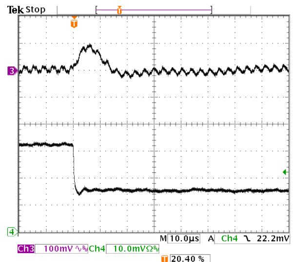
Fig-2.0V-7: Output voltage response for V_{out}=2.0V to positive load current step-change from 6A to 3A with slew rate of -5A/\mu s at V_{in}=5.0V . C_o=47\mu F \times 2 ceramic.
