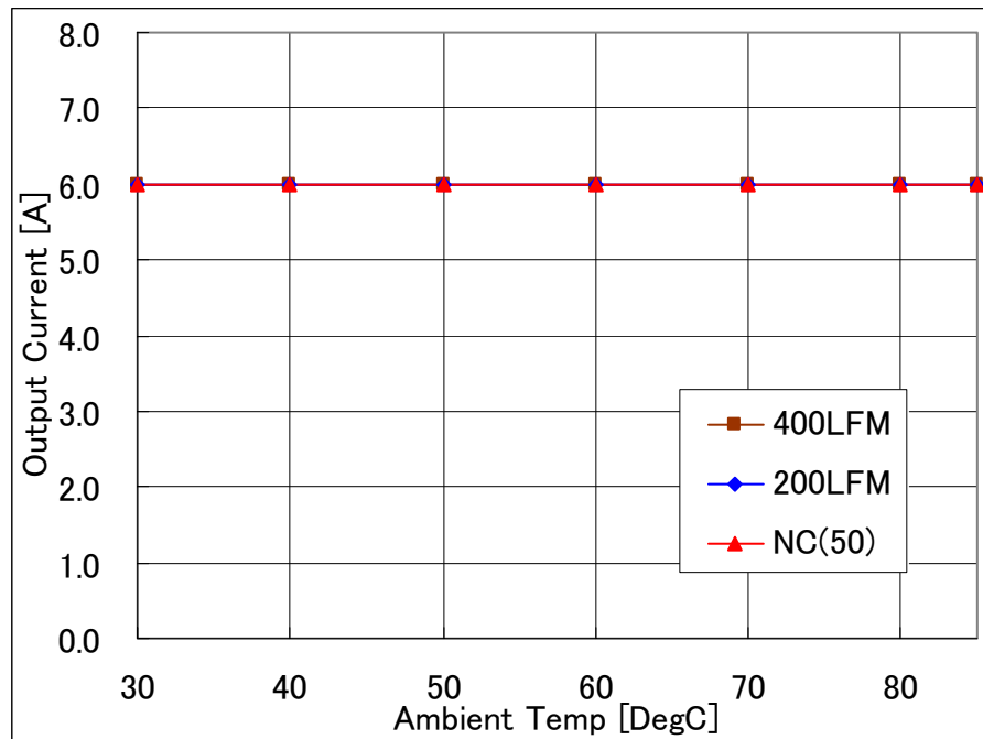
Fig-1.8V-1: Available load current vs. ambient temperature and airflow rates for Vout=1.8V with Vin=5.0V. Maximum component temperature \leq 120^{\circ}\text{C}
