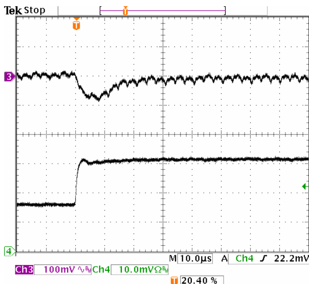
Fig-0.7525V-6: Output voltage response for V_{out}=0.7525V to positive load current step-change from 3A to 6A with slew rate of 5A/\mu s at V_{in}=5.0V . C_o=47\mu F \times 2 ceramic.
