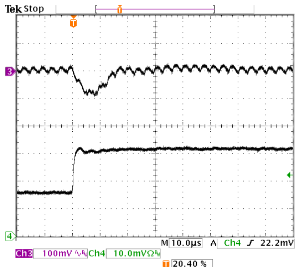
Fig-1.5V-6: Output voltage response for V_{out}=1.5V to positive load current step-change from 3A to 6A with slew rate of 5A/\mu s at V_{in}=5.0V . C_o=47\mu F \times 2 ceramic.
