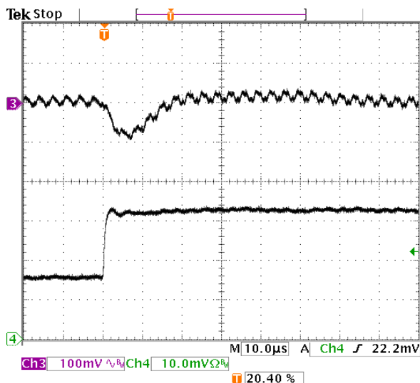
Fig-2.0V-6: Output voltage response for V_{out}=2.0V to positive load current step-change from 3A to 6A with slew rate of 5A/\mu s at V_{in}=5.0V . C_o=47\mu F \times 2 ceramic.
