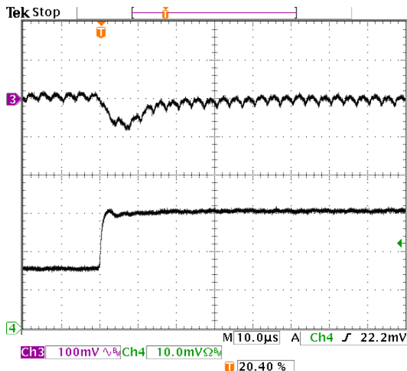
Fig-1.2V-6: Output voltage response for V_{out}=1.2V to positive load current step-change from 3A to 6A with slew rate of 5A/\mu s at V_{in}=5.0V . C_o=47\mu F \times 2 ceramic.
