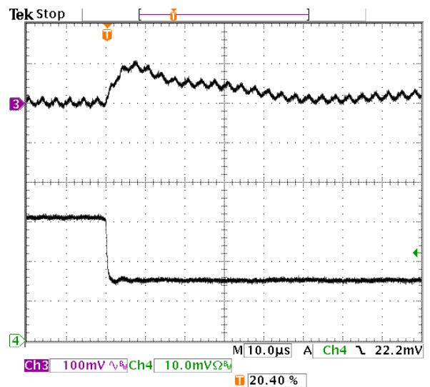
Fig-3.3V-7: Output voltage response for V_{out}=3.3V to negative load current step-change from 6A to 3A with slew rate of -5A/\mu s at V_{in}=5.0V . C_o=47\mu F \times 2 ceramic.
