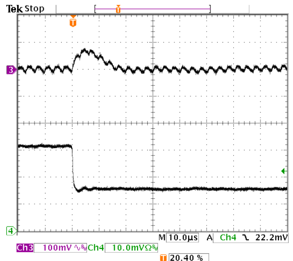
Fig-1.5V-7: Output voltage response for V_{out}=1.5V to positive load current step-change from 6A to 3A with slew rate of -5A/\mu s at V_{in}=5.0V . C_o=47\mu F \times 2 ceramic.
