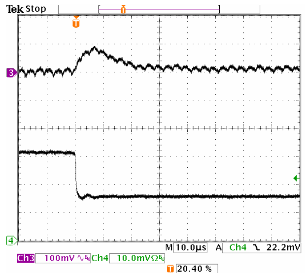
Fig-0.7525V-7: Output voltage response for V_{out}=0.7525V to positive load current step-change from 6A to 3A with slew rate of -5A/\mu s at V_{in}=5.0V . C_o=47\mu F \times 2 ceramic.
