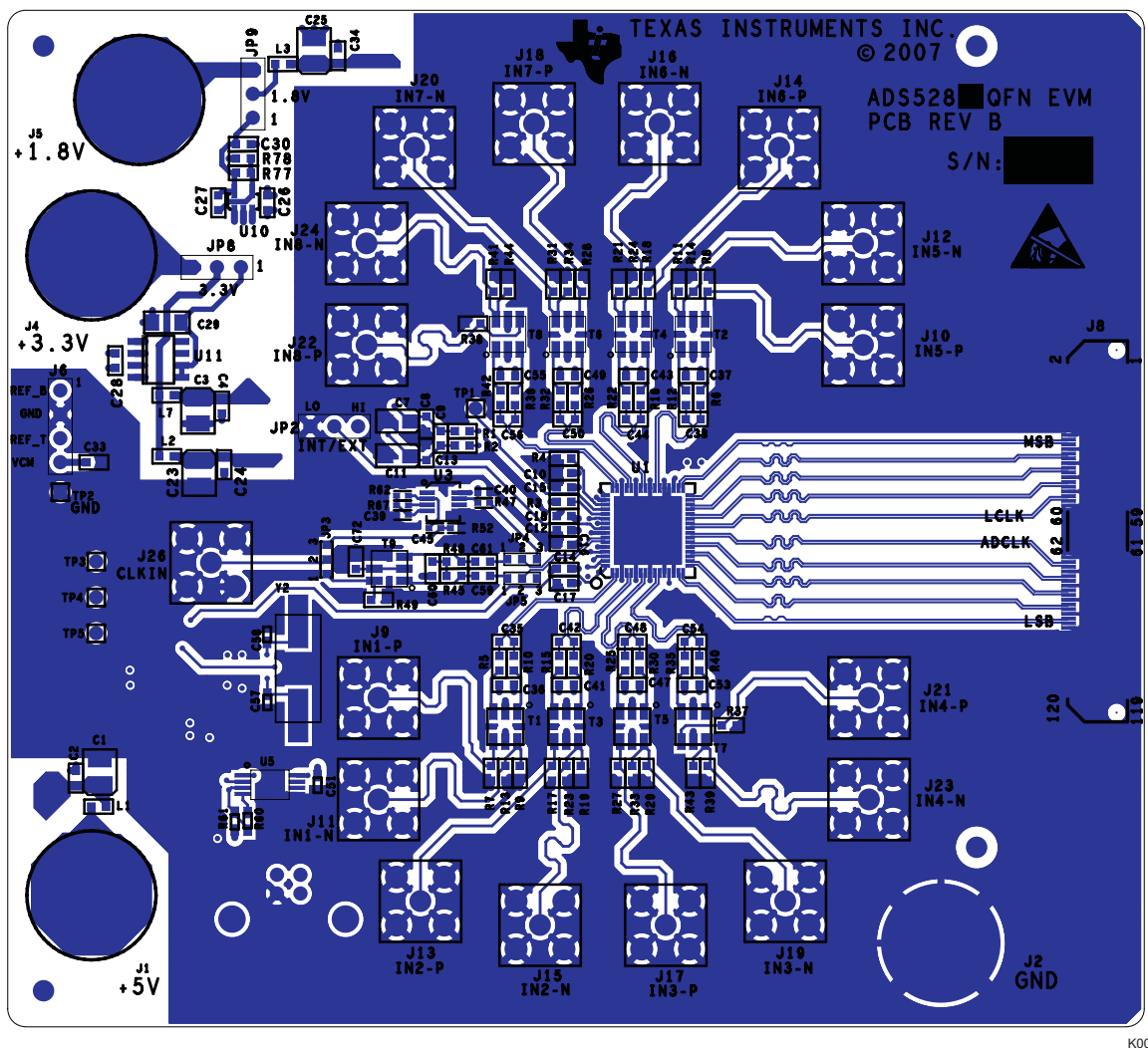
Figure 3. Top Silkscreen
