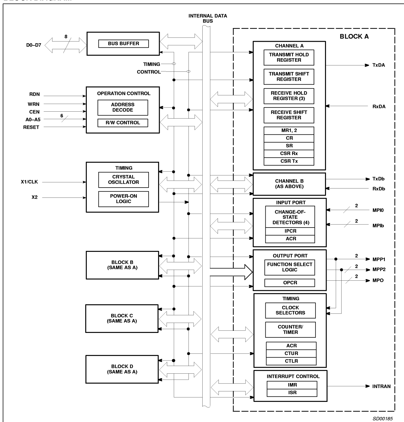
Figure 2. Block Diagram
