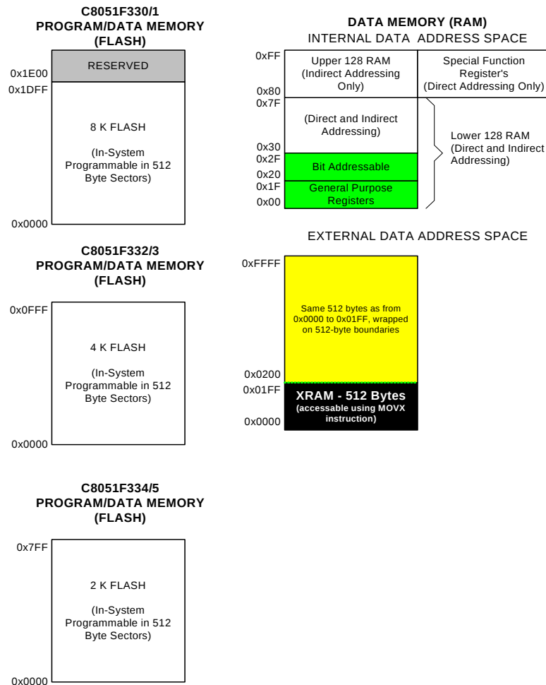
Figure 9.2. Memory Map
