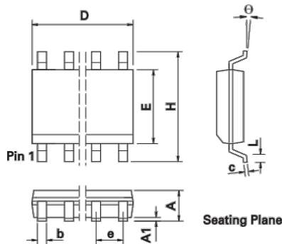
Package details - SO8, SO14
