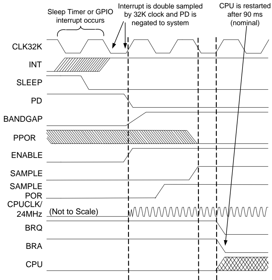
Figure 12. Wakeup Timing
