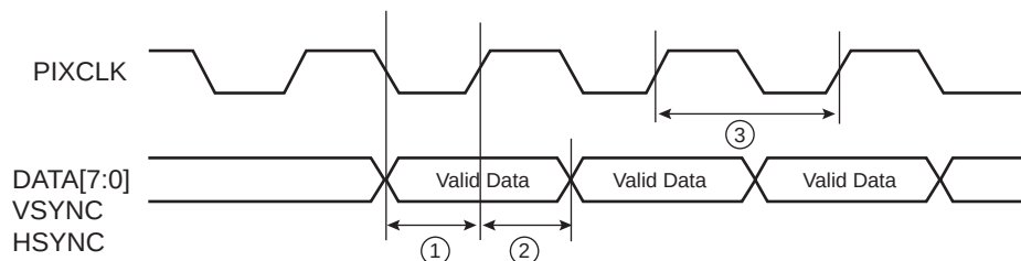
Figure 46-24. ISI Timing Diagram
