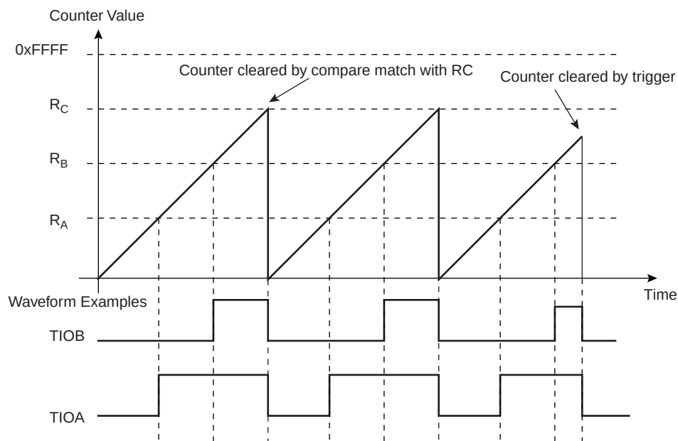
Figure 36-10.WAVSEL = 10 With Trigger
