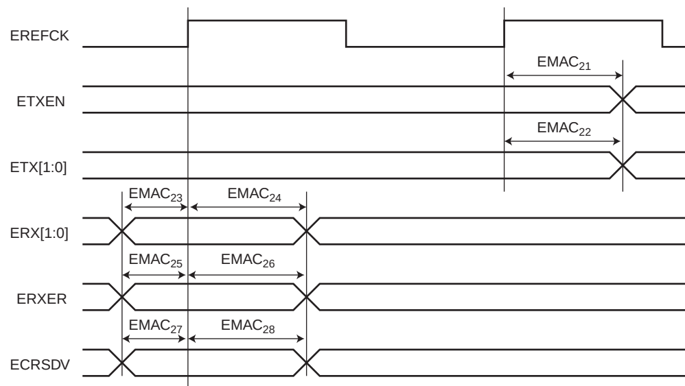
Figure 46-27.EMAC RMII Mode Signals
