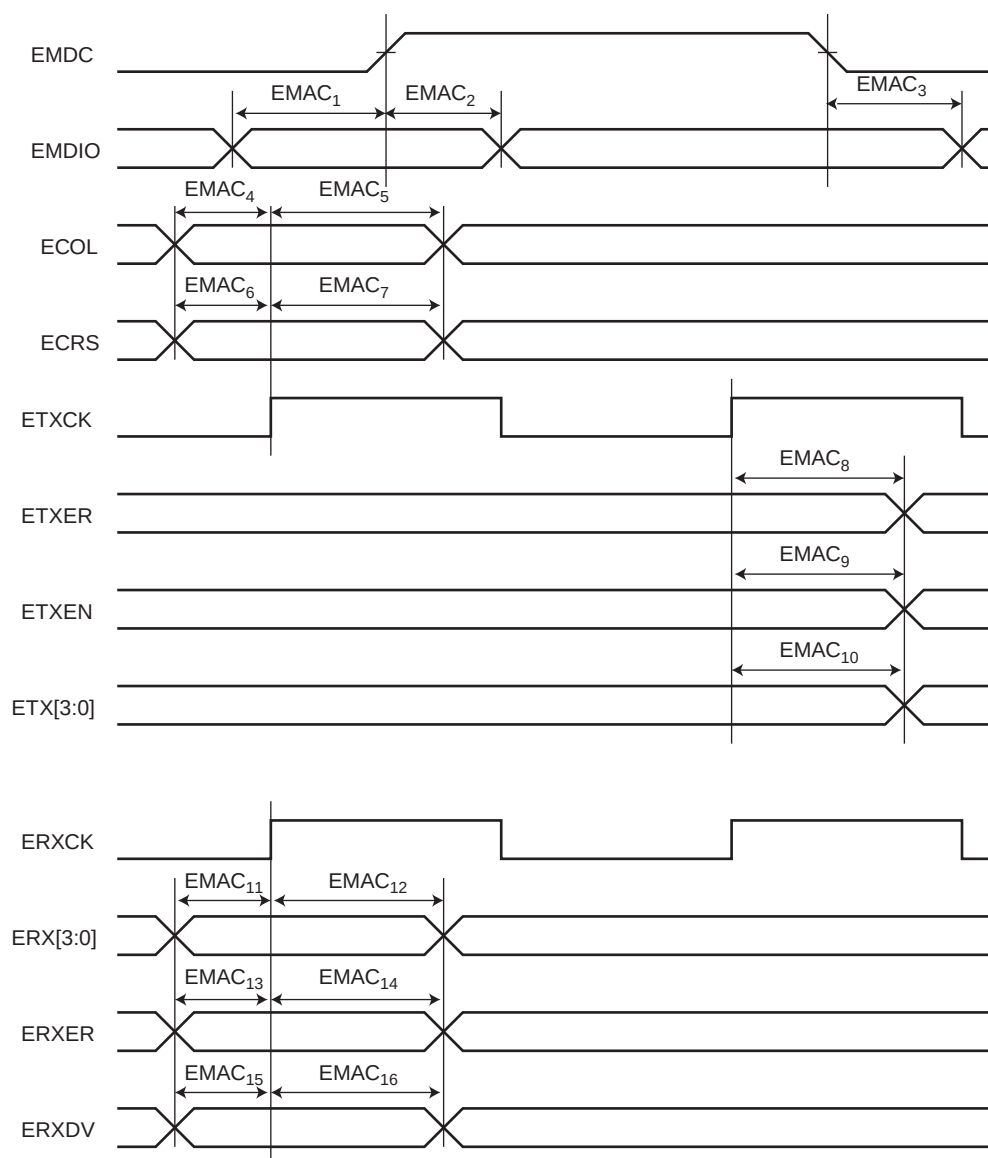
Figure 46-26.EMAC MII Mode Signals
