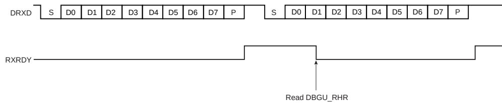
Figure 24-6. Receiver Ready
