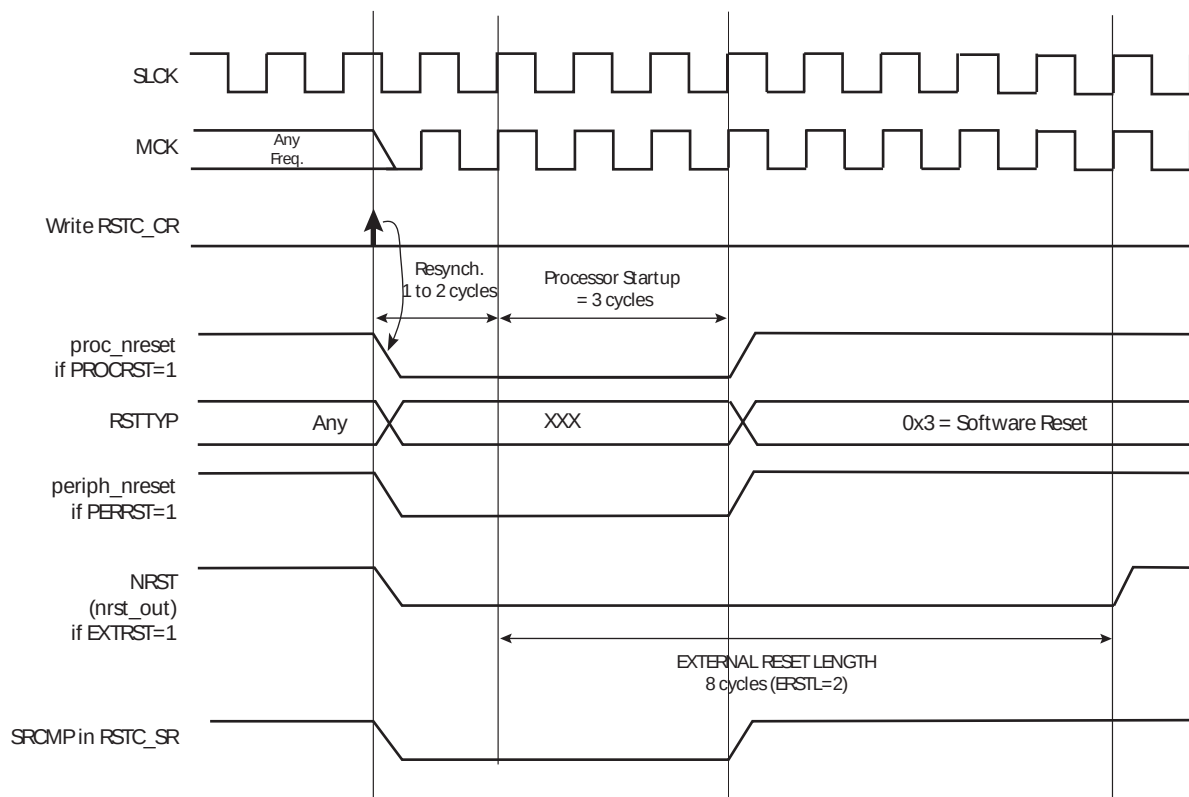
Figure 14-7. Software Reset
