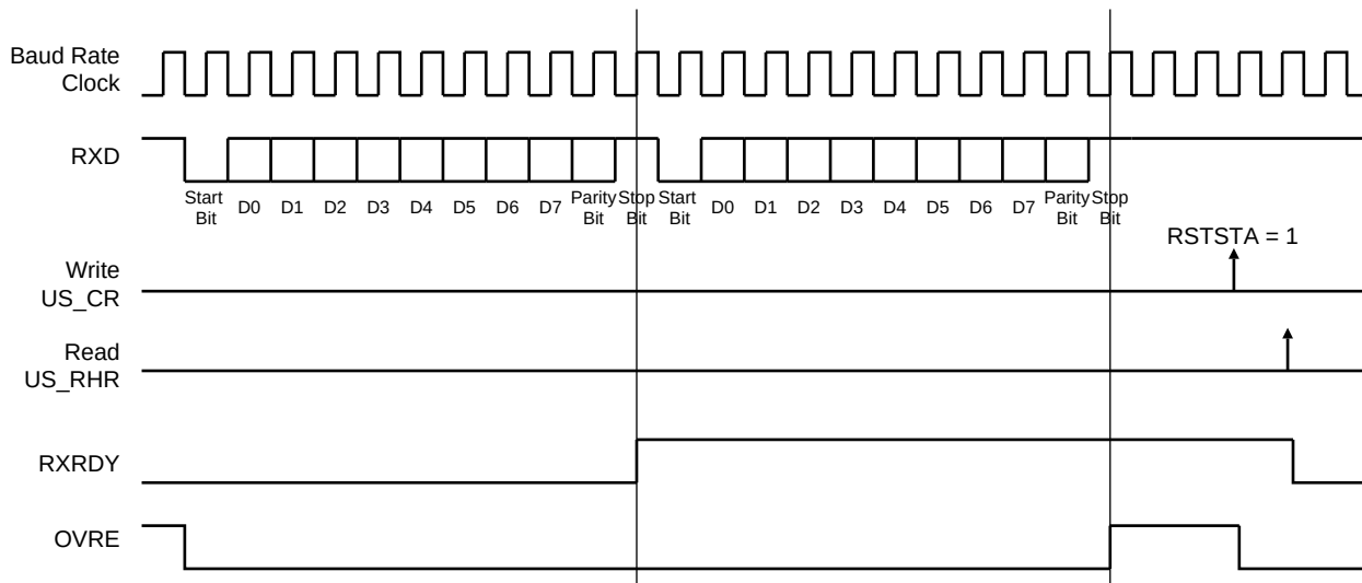
Figure 39-21. Receiver Status
