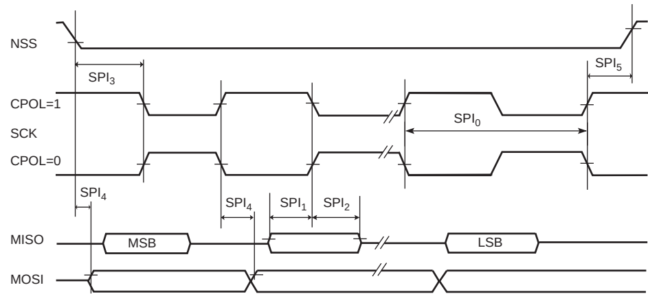
Figure 46-28.USART SPI Master Mode
