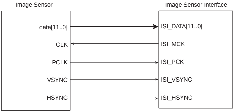
Figure 44-1. ISI Connection Example
