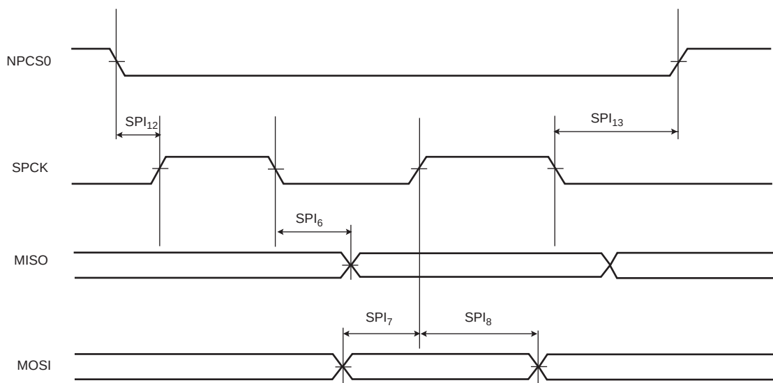
Figure 46-11.SPI Slave mode 0 and 3
