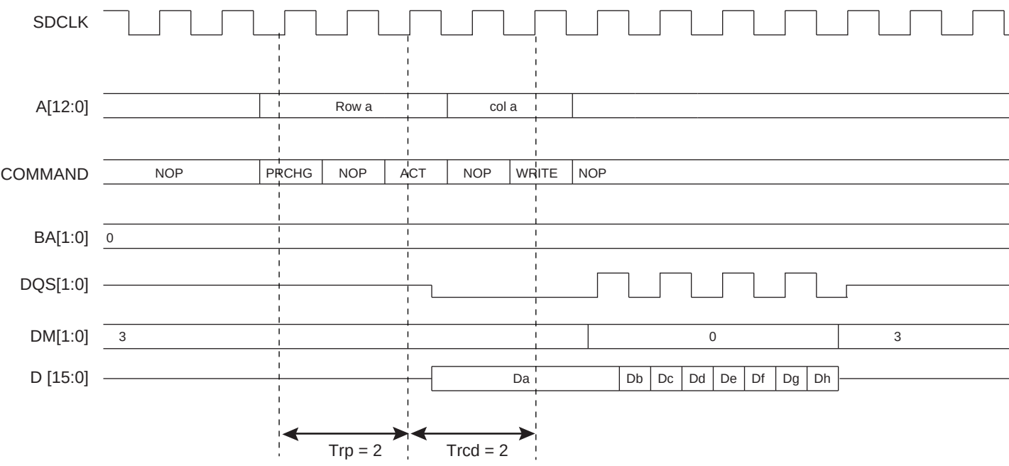
Figure 30-5. Burst Write Access, Row Closed, Low-power DDR1-SDRAM Device
