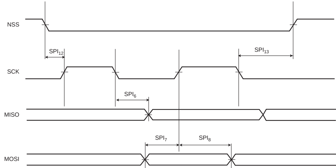
Figure 46-29.USART SPI Slave mode: (Mode 1 or 2)
