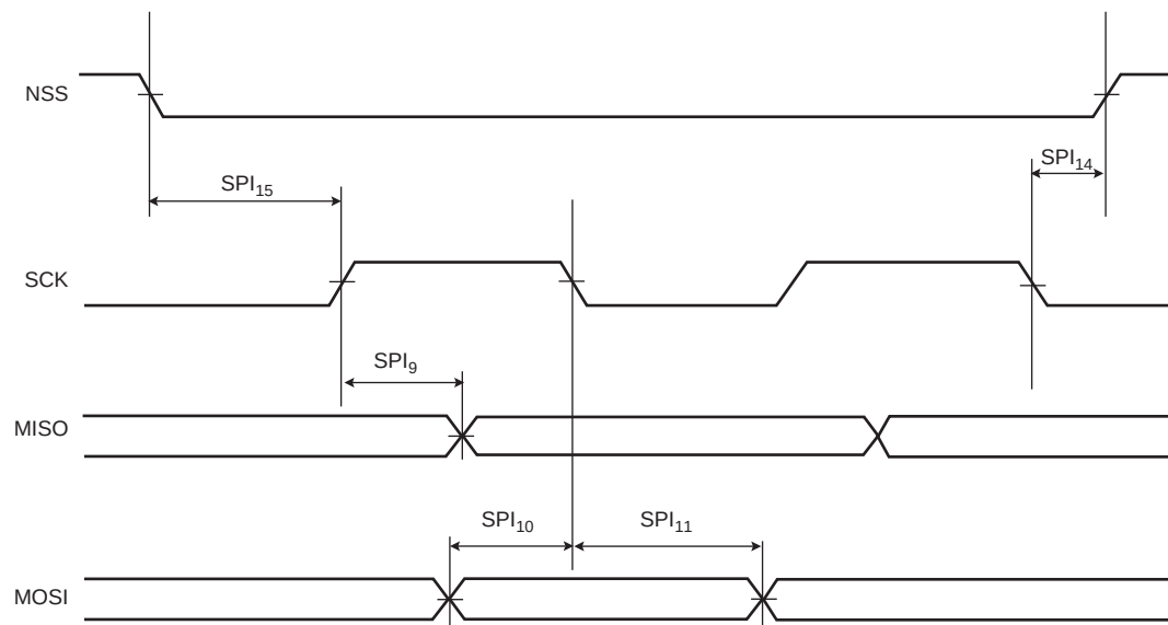
Figure 46-30.USART SPI Slave mode: (Mode 0 or 3)
