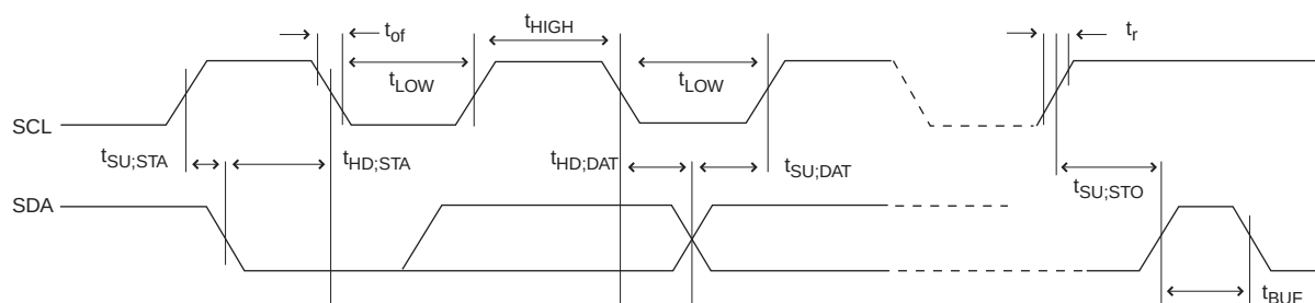
Figure 46-31. Two-wire Serial Bus Timing
