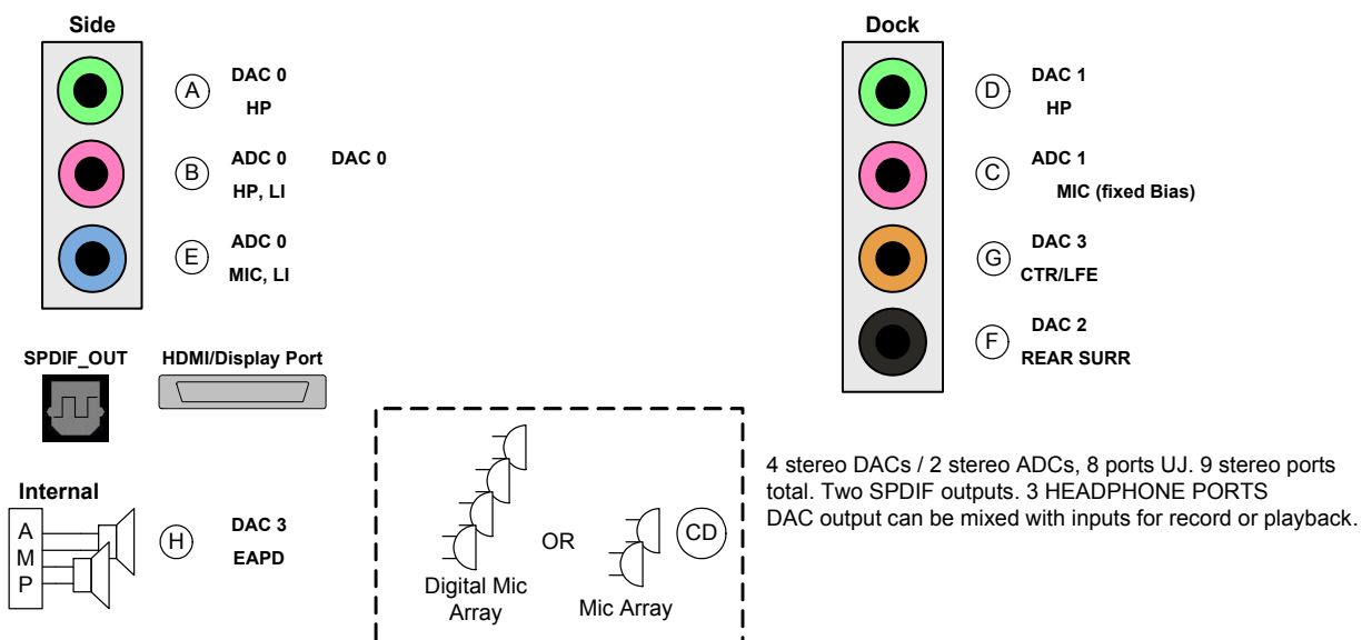
Figure 13. Port Configurations
