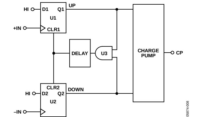
Figure 14. PFD Simplified Schematic
