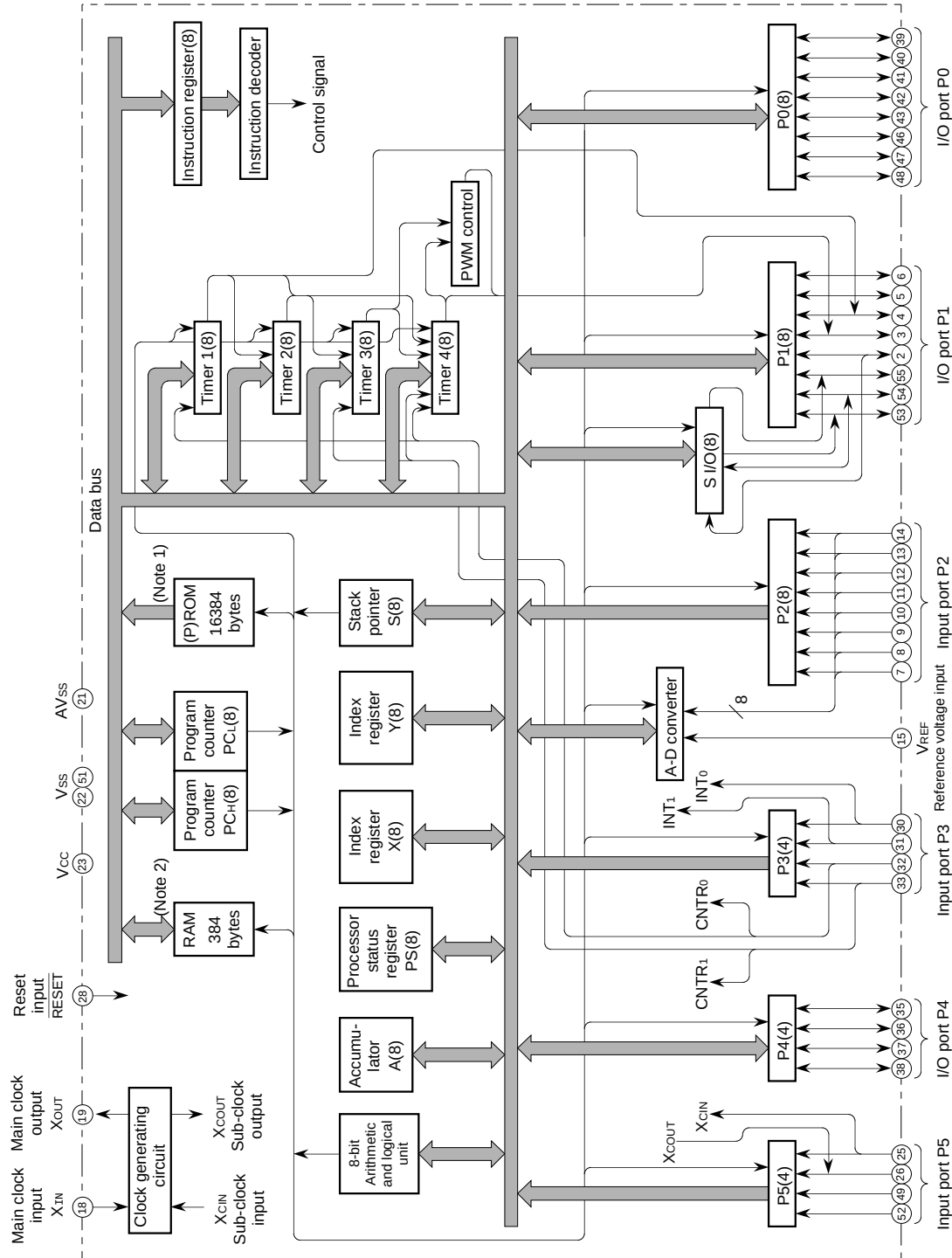
M37478M8/E8-XXXXFP, M37478M8/E8TXXXXFP BLOCK DIAGRAM
