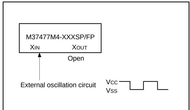
Fig. 25 External clock input circuit (7477 group)
