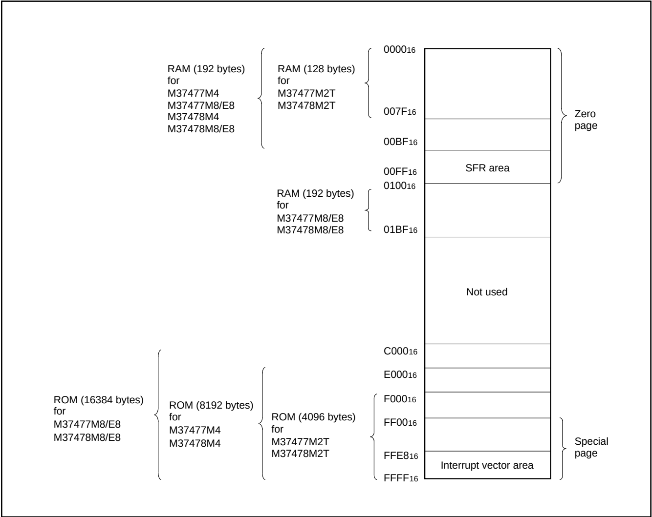
Fig. 2 Memory map
