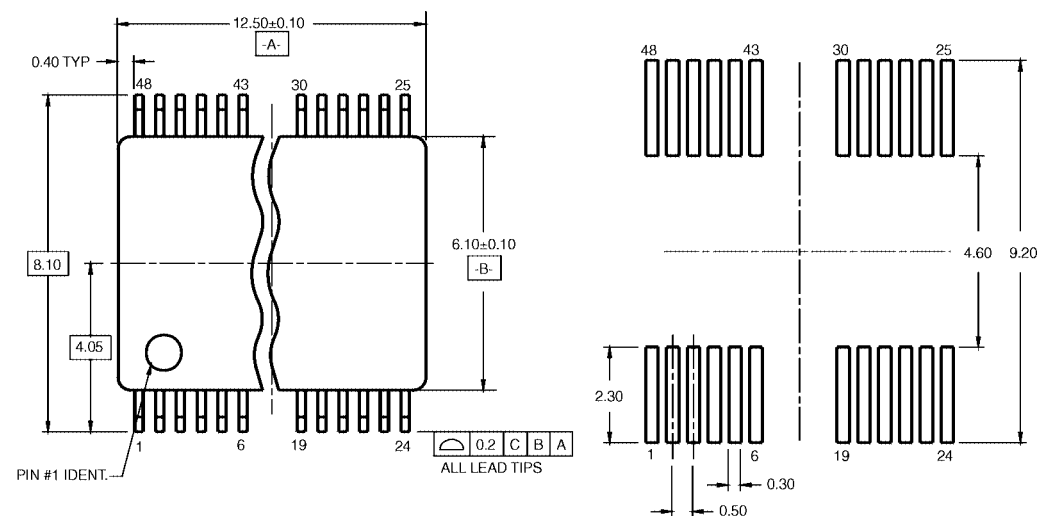
LAND PATTERN RECOMMENDATION
