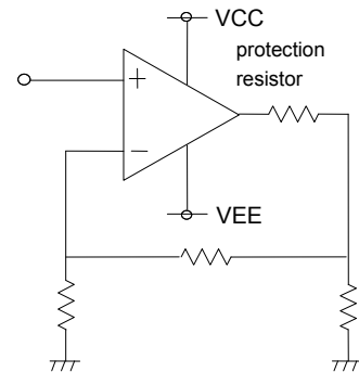
Fig. 322 The example of output short protection
