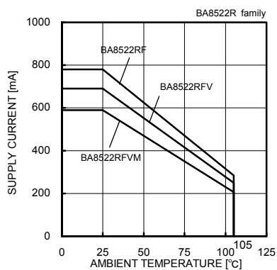
Fig. 177 Derating Curve
