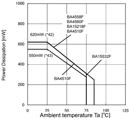
(e)BA4558/BA4560/BA15218/BA15532/BA4510 family
