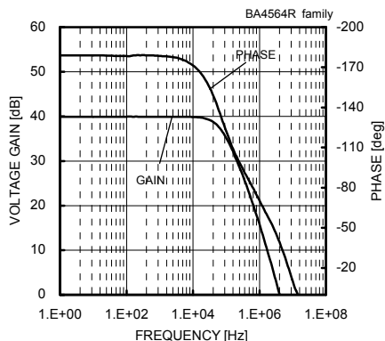
Fig. 110 Voltage Gain - Frequency ( V_{CC}/V_{EE}=+15[V]/-15[V] , A_v=40[dB] , R_L=2[k\Omega] , T_a=25[°C] )
