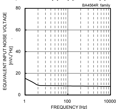
Fig. 107 Equivalent Input Noise Voltage - Frequency ( V_{CC}/V_{EE}=+15[V]/-15[V] , R_s=100[\Omega] , T_a=25[°C] )
