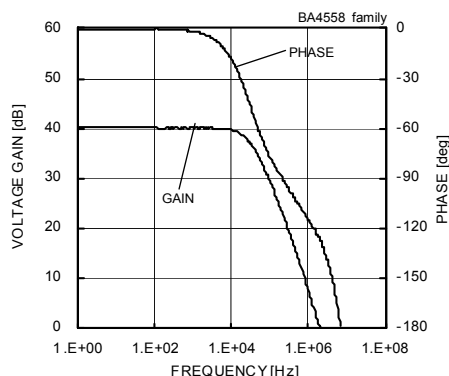
Fig.22 Voltage Gain - Frequency ( V_{CC}/V_{EE}=+15[V]/-15[V] , A_v=40[dB] , R_L=2[k\Omega] , T_a=25[^\circ C] )
