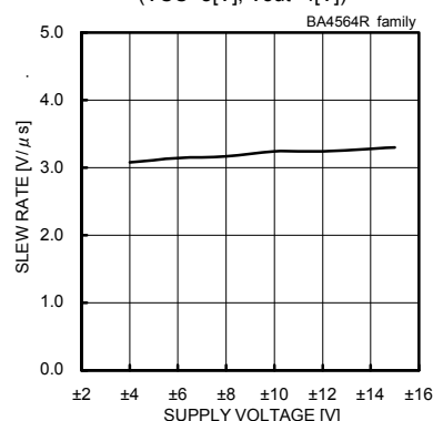
Fig. 106 Slew Rate - Supply Voltage ( C_L=100[pF] , R_L=2[k\Omega] , T_a=25[°C] )
