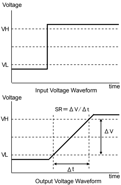
Fig. 317 Slew rate input output wave
