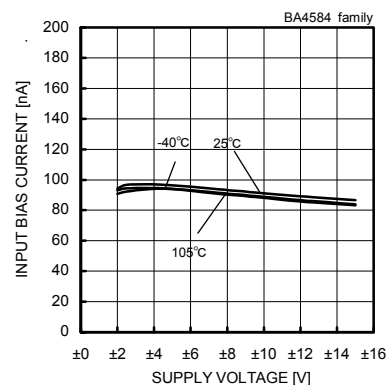
Fig. 143 Input Bias Current - Supply Voltage (Vicm=0[V], Vout=0[V])
