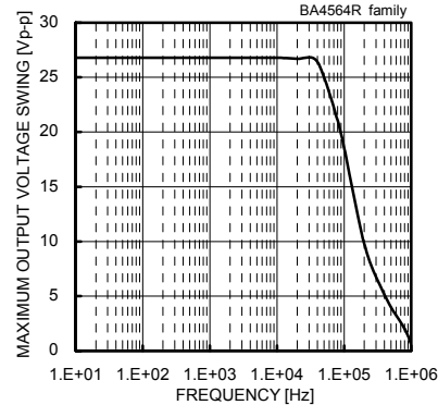
Fig. 109 Maximum Output Voltage Swing - Frequency ( V_{CC}/V_{EE}=+15[V]/-15[V] , R_L=2[k\Omega] , T_a=25[°C] )
