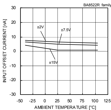
Fig. 190 Input Offset Current - Ambient Temperature ( V_{icm}=0[V] , V_{out}=0[V] )
