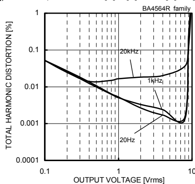
Fig. 108 Total Harmonic Distortion - Output Voltage ( V_{CC}/V_{EE}=+15[V]/-15[V] , A_v=20[dB] , R_L=2[k\Omega] , 80[kHz] -LPF, T_a=25[°C] )
