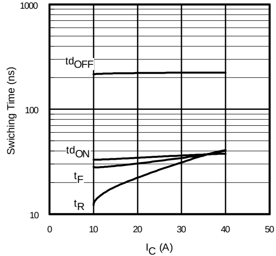
Fig. 14 - Typ. Switching Time vs. I_C T_J = 150^\circ C ; L=200\mu H ; V_{CE} = 400V R_G = 22\Omega ; V_{GE} = 15V
