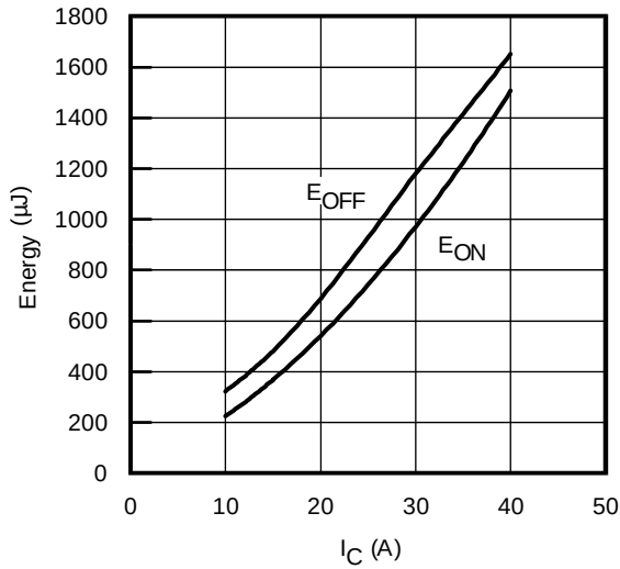
Fig. 13 - Typ. Energy Loss vs. I_C T_J = 150^\circ C ; L=200\mu H ; V_{CE} = 400V R_G = 22\Omega ; V_{GE} = 15V
