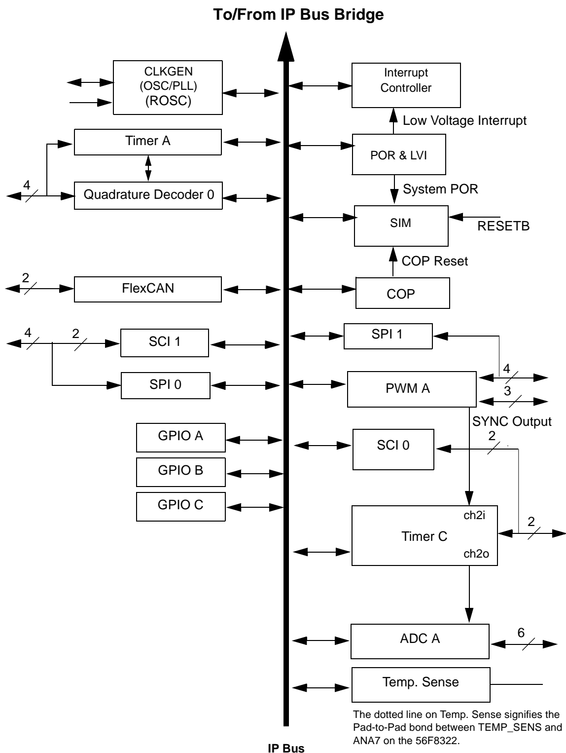
Figure 1-2 Peripheral Subsystem
