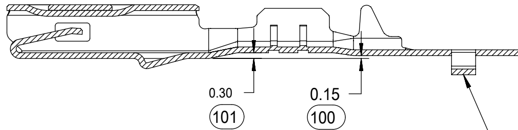
SECTION AA-AA M3 GRIP CODE TERMINAL SEE TABLE (SHEET 2) FOR PART NUMBERS
