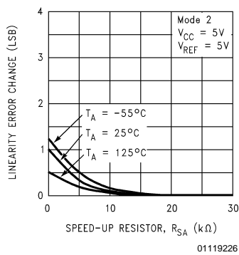
Linearity Change vs Speed-Up Resistor
