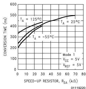
Conversion Time vs Speed-Up Resistor
