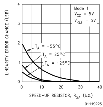
Linearity Change vs Speed-Up Resistor
