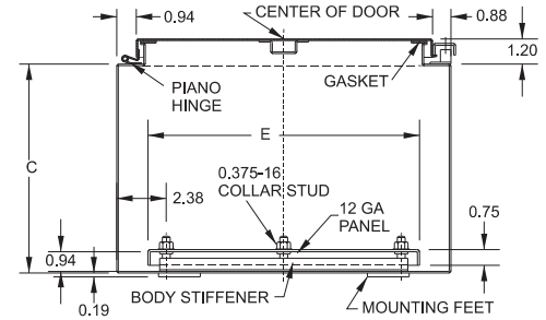
Section Y-Y
