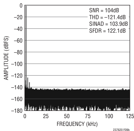
Figure 9b. 128k Point FFT Plot with f_{IN} = 2\text{kHz} for Circuit Shown in Figure 9a
