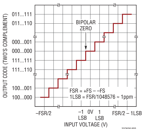
Figure 2. LTC2376-20 Transfer Function
