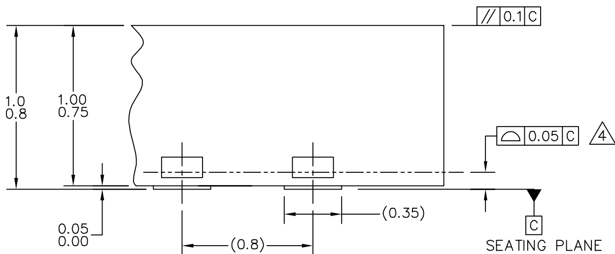
DETAIL G
