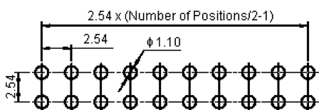
PCB Layout
