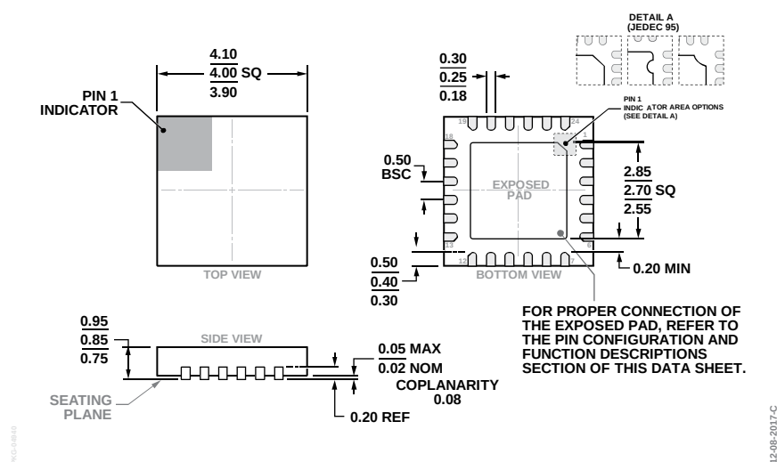
Figure 101. 24-Lead Lead Frame Chip Scale Package [LFCSP], 4 mm × 4 mm Body and 0.85 mm Package Height (HCP-24-3)
