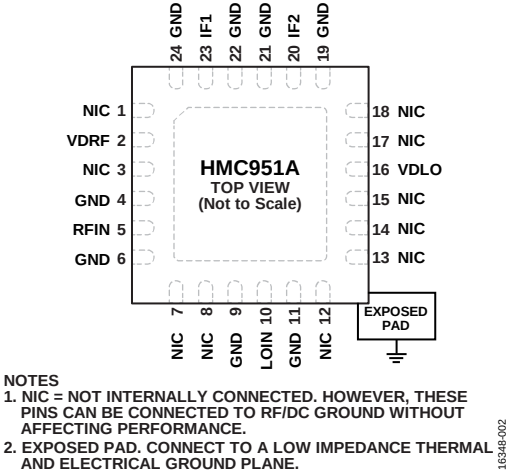
Figure 2. Pin Configuration
