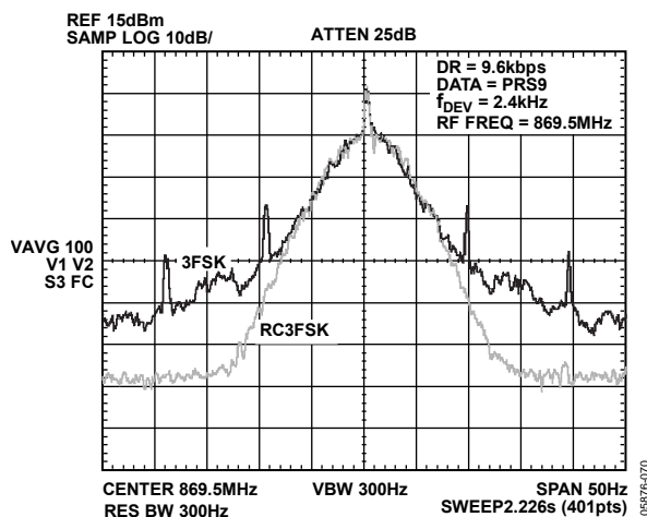
Figure 17. Output Spectrum in 3FSK and Raised Cosine 3FSK Modes
