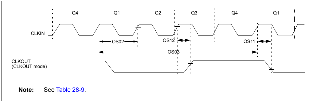
FIGURE 28-5: CLOCK TIMING
