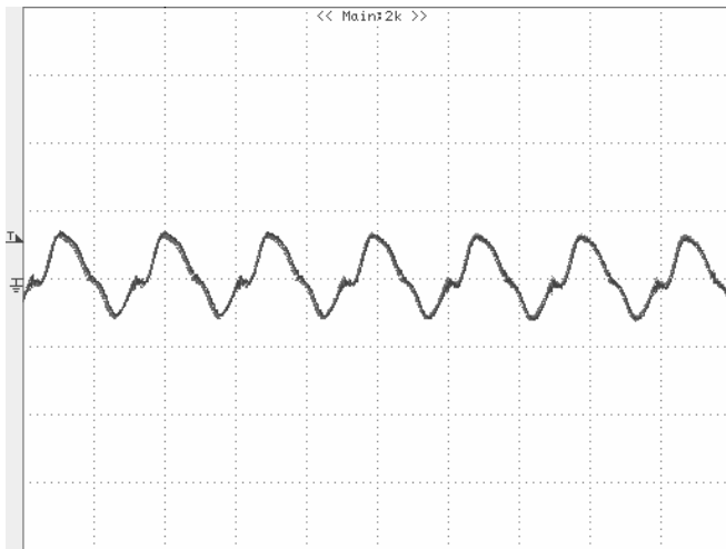
Figure 14: Output voltage ripple at nominal input voltage and rated load current ( I_o=20A ) (20 mV/div, 2 \mu s/div) Load capacitance: 1 \mu F ceramic capacitor and 10 \mu F tantalum capacitor. Bandwidth: 20 MHz. Scope measurements should be made using a BNC cable (length shorter than 20 inches). Position the load between 51 mm to 76 mm (2 inches to 3 inches) from the module
