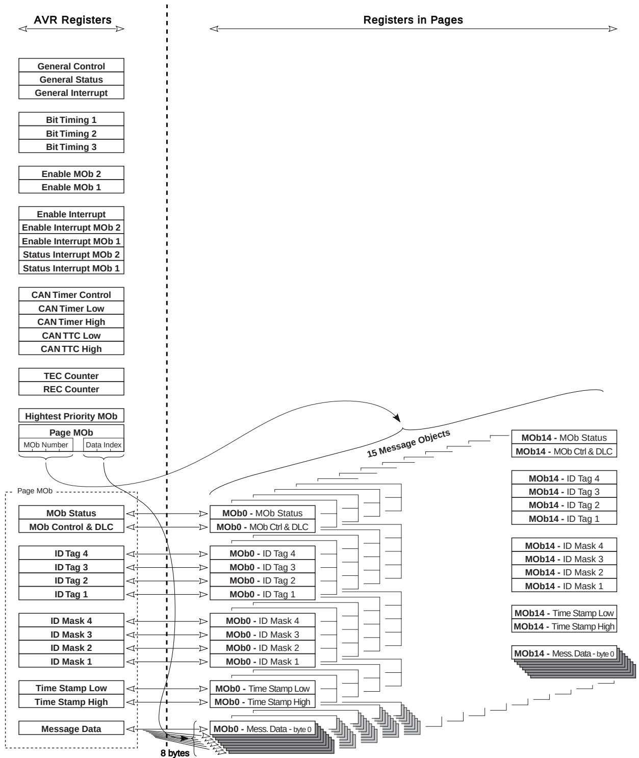
Figure 125. Registers Organization
