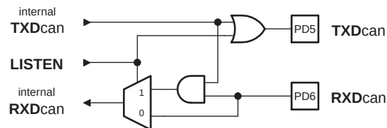
Figure 116. Listening Mode
