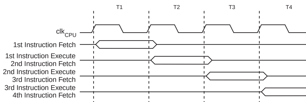
Figure 7. The Parallel Instruction Fetches and Instruction Executions
