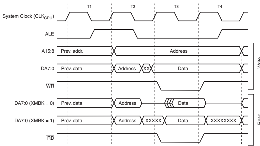
Figure 14. External Data Memory Cycles no Wait-state (SRWn1=0 and SRWn0=0) (1)
