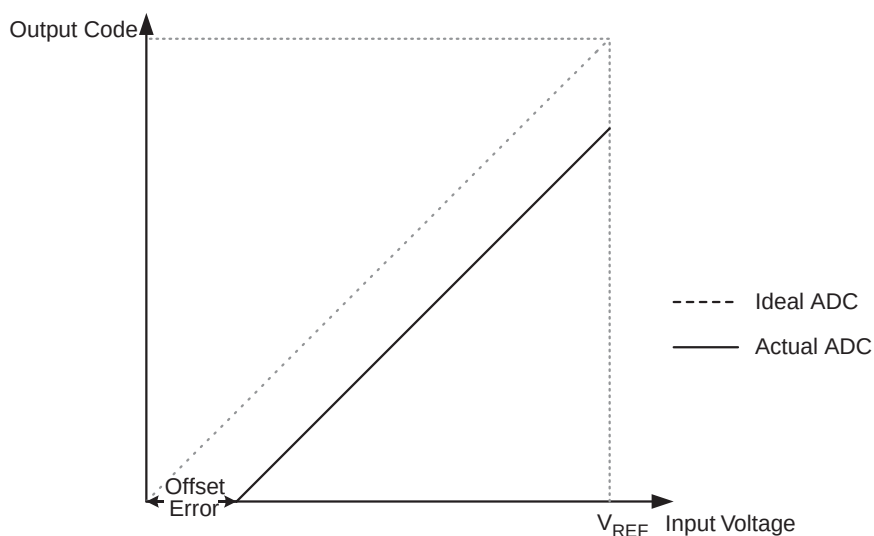
Figure 136. Offset Error
