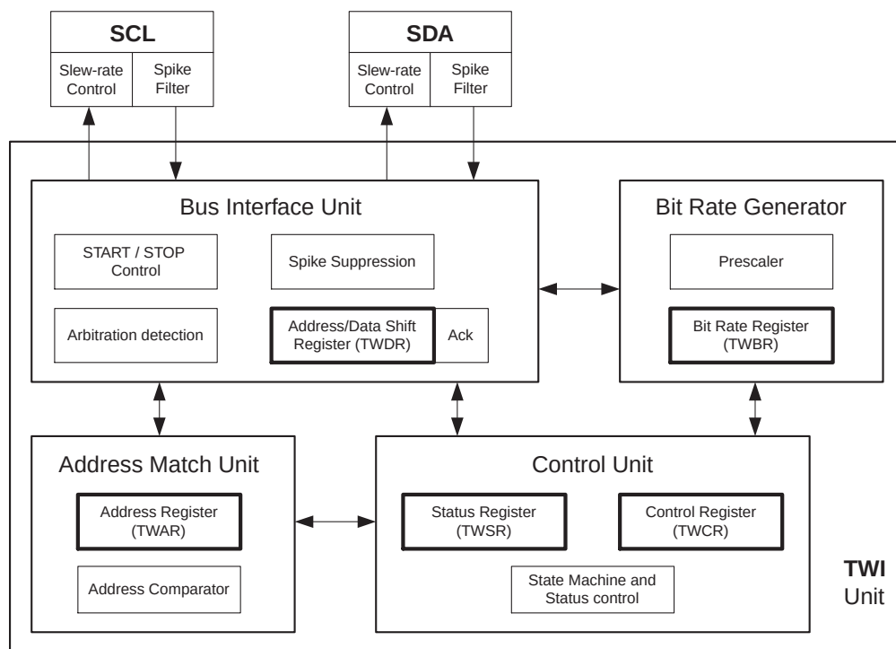
Figure 98. Overview of the TWI Module
