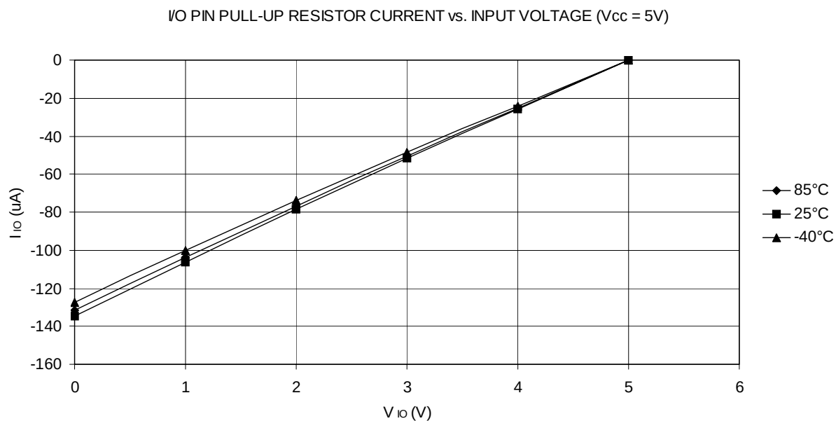
Figure 194. I/O Pin Pull-up Resistor Current vs. Input Voltage (Vcc = 5V)
