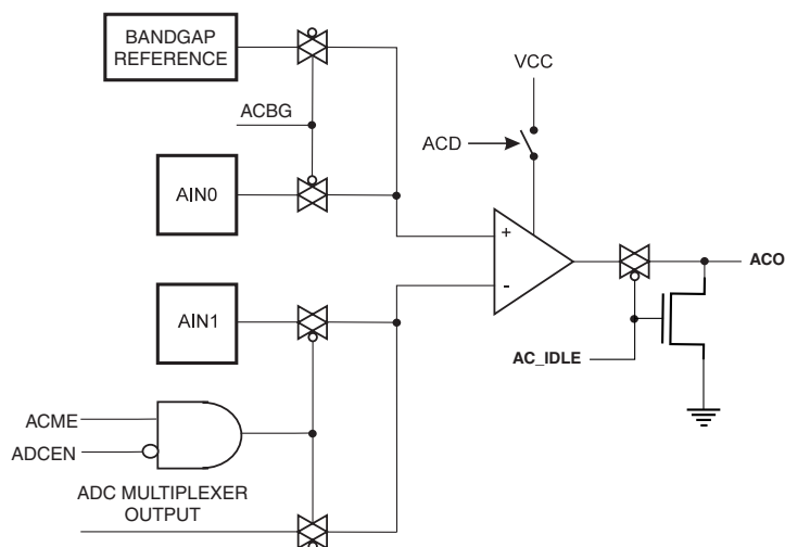
Figure 150. Analog Comparator
