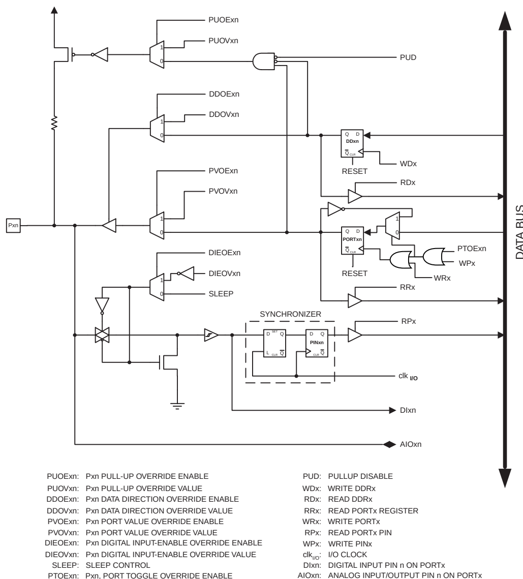
Figure 34. Alternate Port Functions (1)
