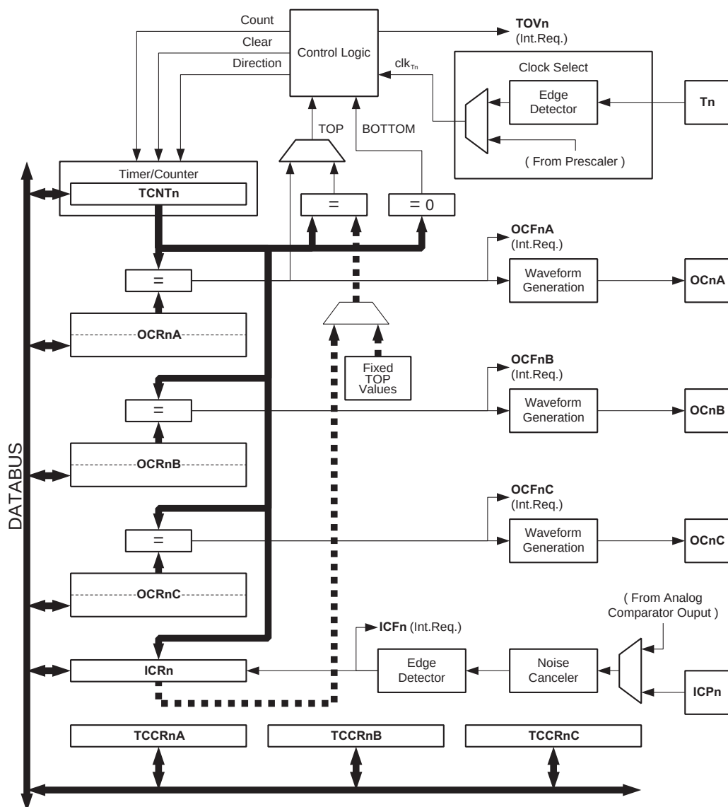
Figure 48. 16-bit Timer/Counter Block Diagram (1)
