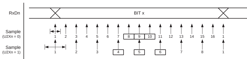
Figure 88. Sampling of Data and Parity Bit
