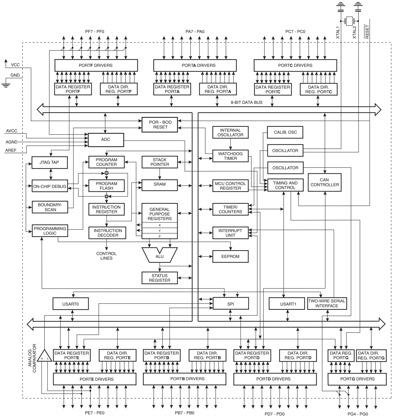
Figure 1. Block Diagram
