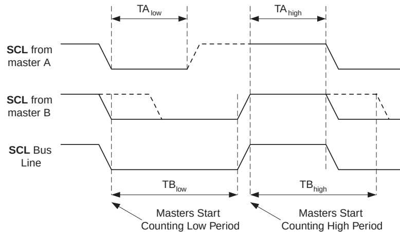
Figure 96. SCL Synchronization between Multiple Masters
