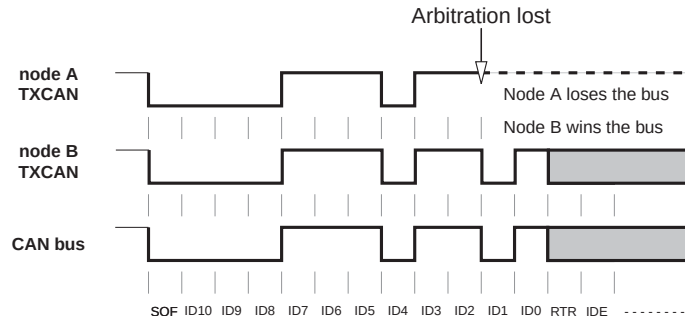
Figure 114. Bus Arbitration
