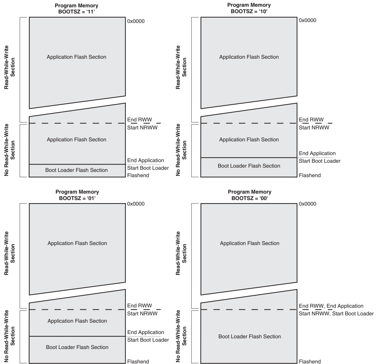
Figure 154. Memory Sections
