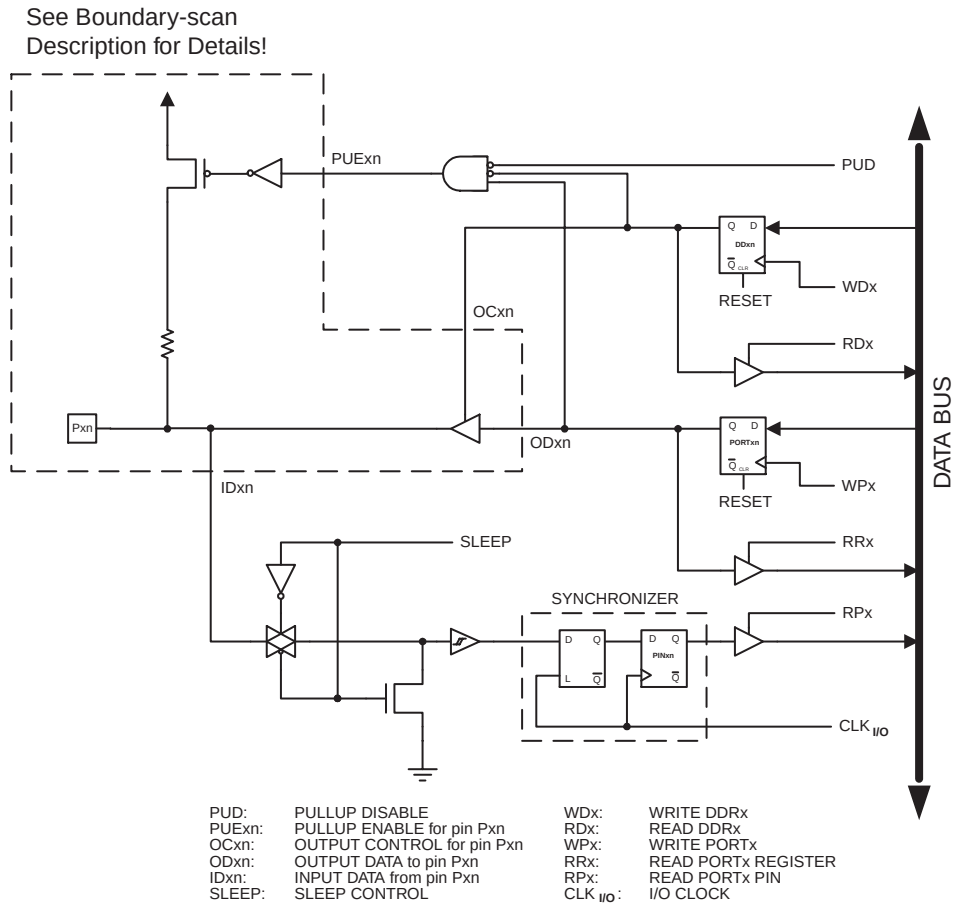
Figure 146. General Port Pin Schematic Diagram
