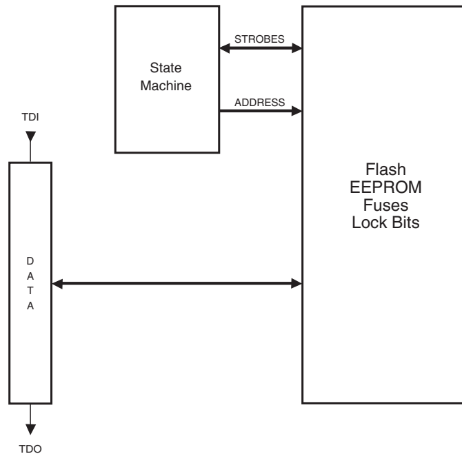
Figure 168. Flash Data Byte Register
