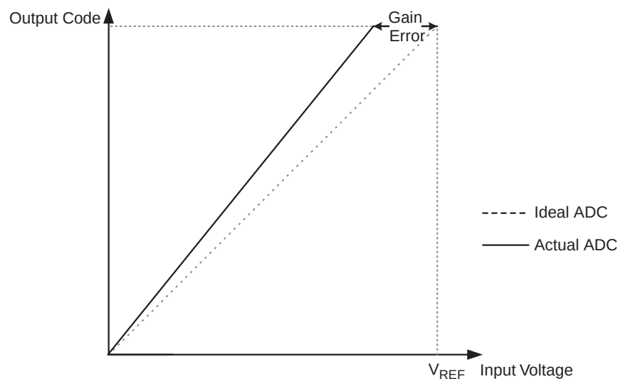
Figure 137. Gain Error
