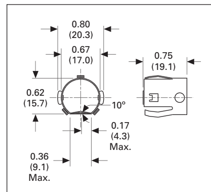
Figure 11-52. #006-10478 Front Mount Clip
