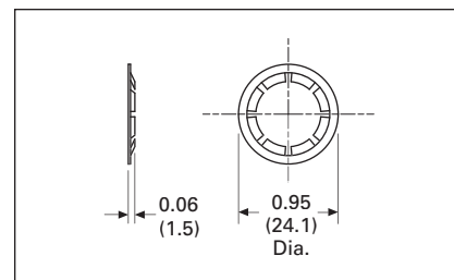
Figure 11-51. #006-10417 Retaining Ring
