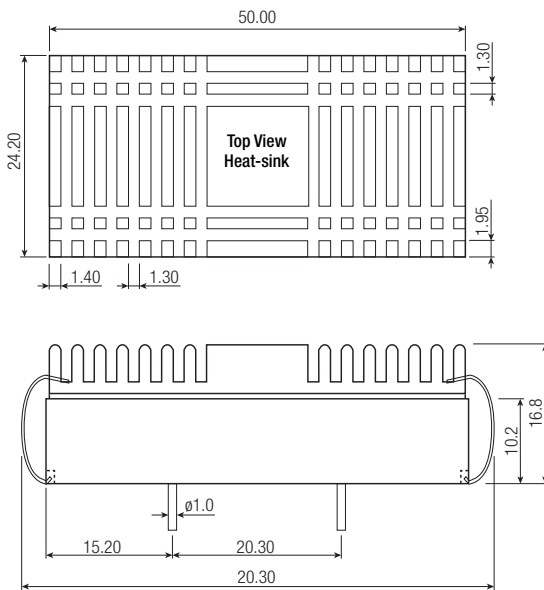
Dimension Drawing (mm) with Heat-sink
