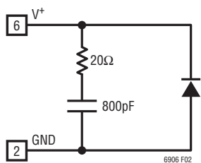
Figure 2. V+ Pin
