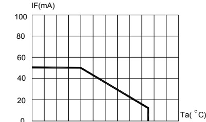
FIG.4a RED MAXIMUM FORWARD DC CURRENT VS AMBIENT TEMPERATURE ( T_{jmax}=105^{\circ}\text{C} )
