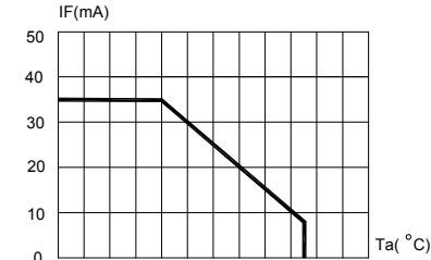
FIG.4b BLUE & GREEN MAXIMUM FORWARD DC CURRENT VS AMBIENT TEMPERATURE ( T_{jmax}=105^{\circ}\text{C} )
