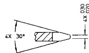
PARTIAL SECTION A-A
