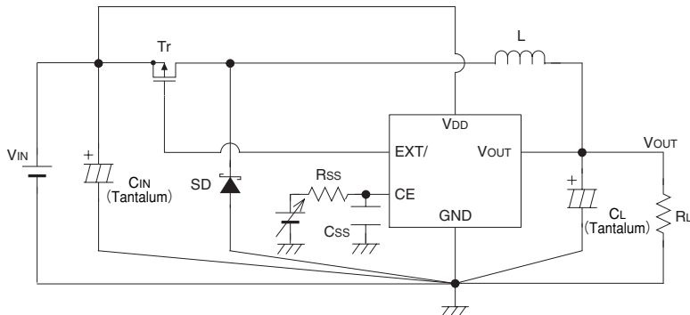
Circuit 3. XC6365C, XC6366C
