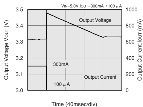
XC6366A333MR (300kHz,3.3V)
