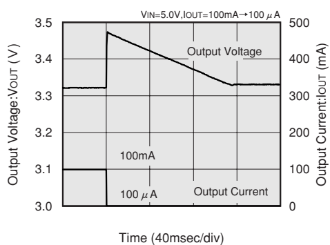
XC6366A333MR (300kHz,3.3V)
