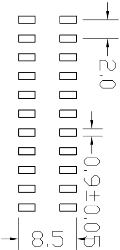
PCB LAYOUT
