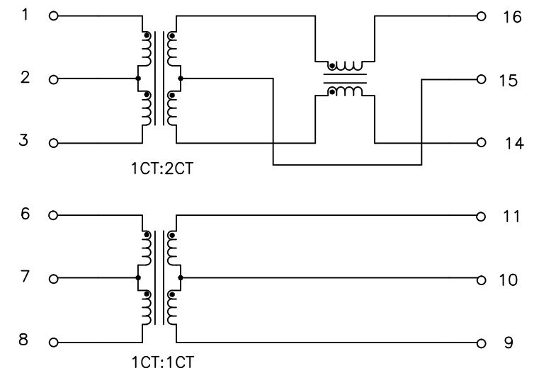
SCHEMATIC
