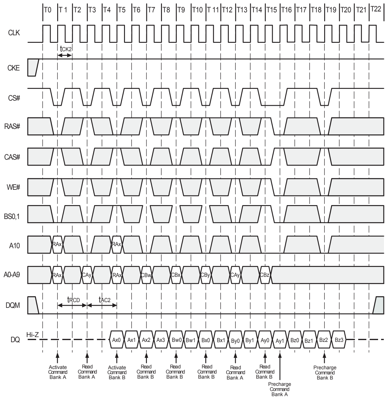
Figure 14.2. Interleaving Column Read Cycle (Burst Length=4, CAS# Latency=2)
