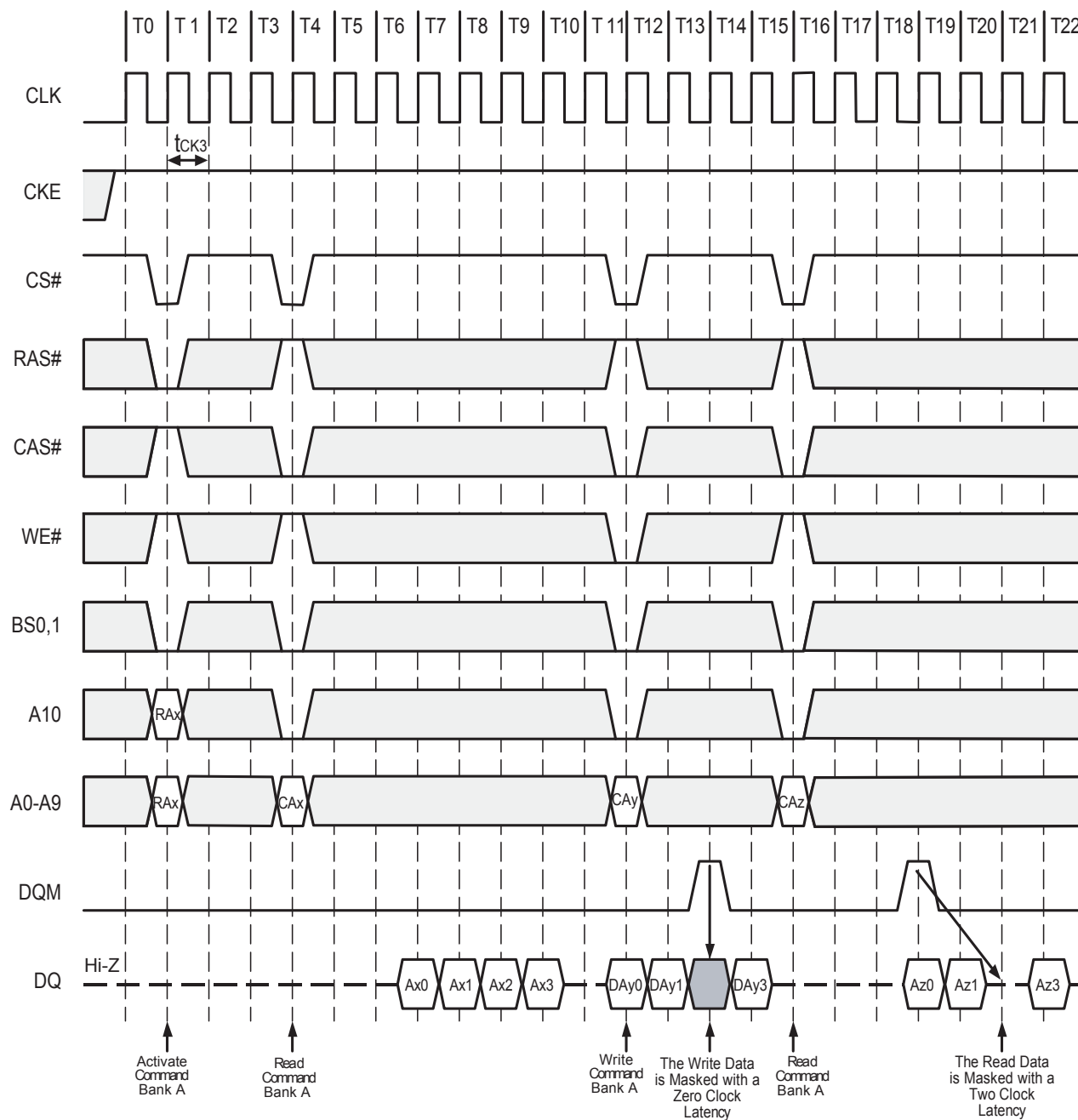
Figure 13.3. Read and Write Cycle (Burst Length=4, CAS# Latency=3)
