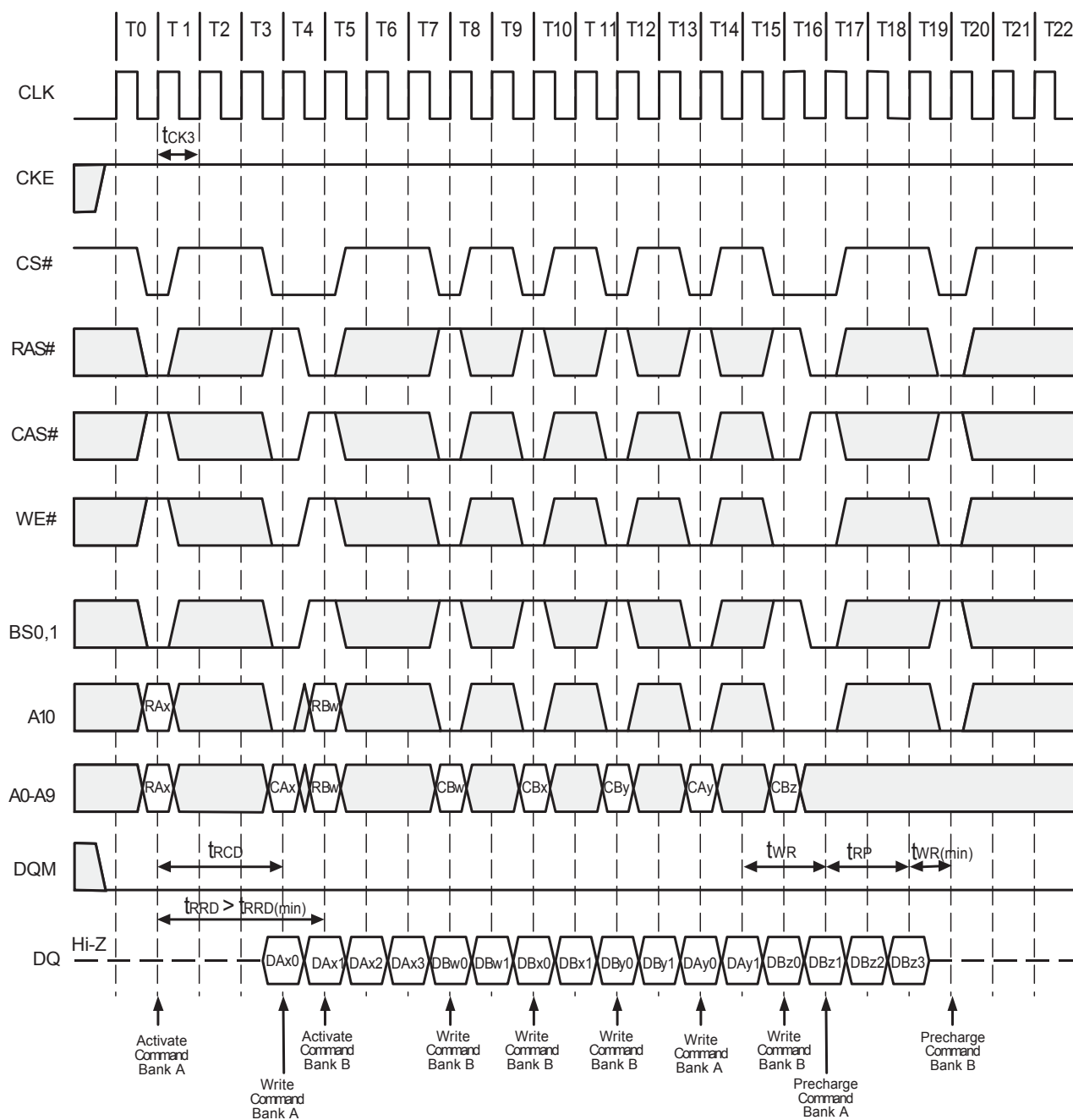
Figure 15.3. Interleaved Column Write Cycle (Burst Length=4, CAS# Latency=3)
