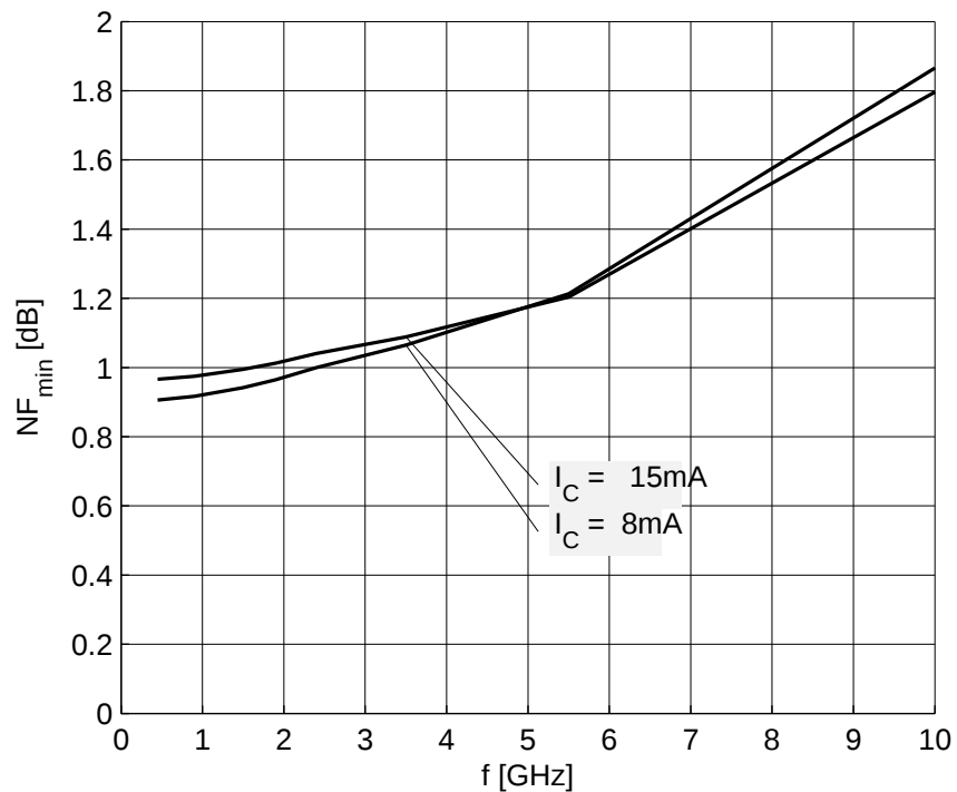
Figure 7-10 Noise Figure NF_{\min} = f(f) , V_{CE} = 1.8 \text{ V} , I_C = 8 / 15 \text{ mA} , Z_S = Z_{\text{opt}}
