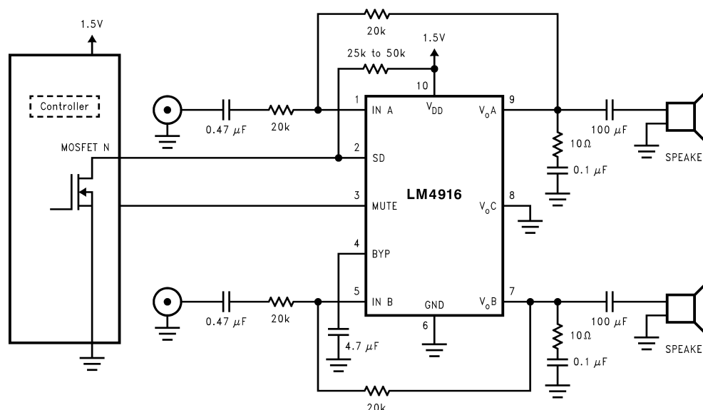
Figure 38. Recommended Circuit for Different Supply Turn-On Timing
