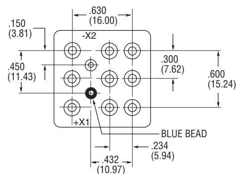
TERMINAL VIEW
