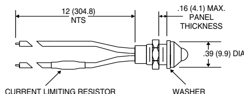
PH31 Dimensions
