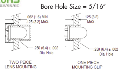
PH25 Mounting
