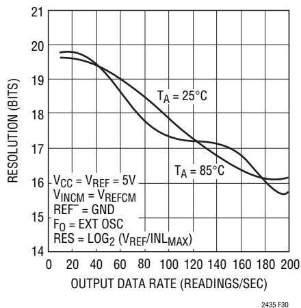
Figure 30. Resolution ( INLRMS \leq 1LSB ) vs Output Data Rate and Temperature
