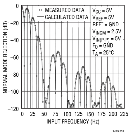
Figure 39. Input Normal Mode Rejection vs Input Frequency with Running Average
