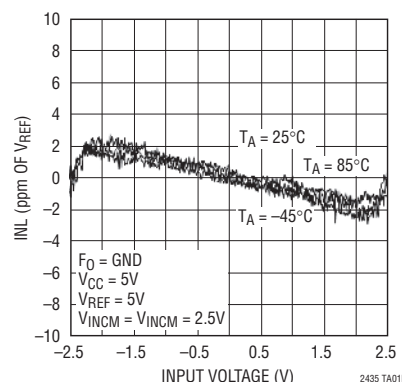
Integral Nonlinearity vs Input
