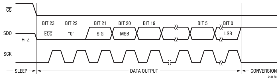
Figure 3. Output Data Timing
