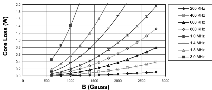
Core Loss vs. Flux Density HM69-60R10LFTR
