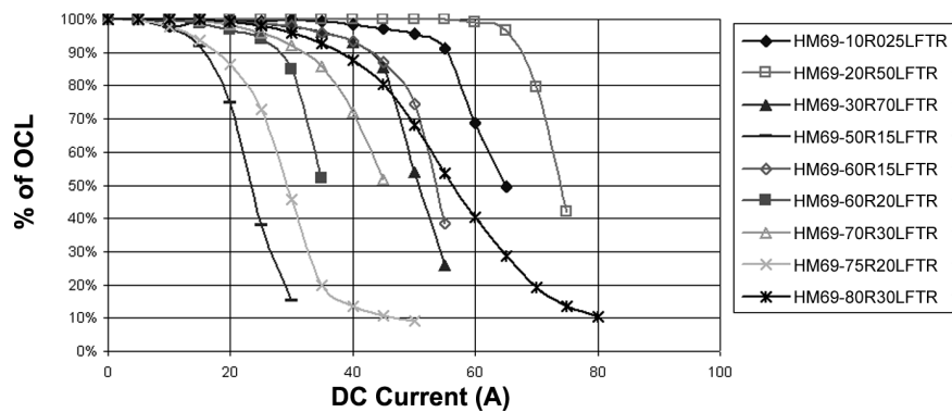
Inductance Rolloff vs. Current Characteristics
