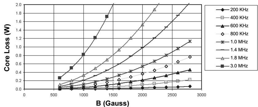
Core Loss vs. Flux Density HM69-55R10LFTR
