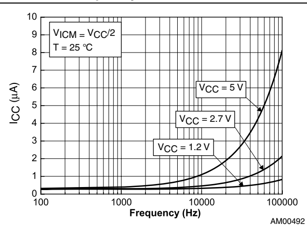
Figure 7. Current consumption vs. toggle frequency
