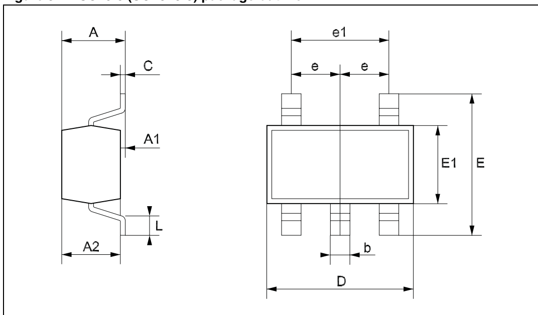
Figure 34. SC70-5 (SOT323-5) package outline
