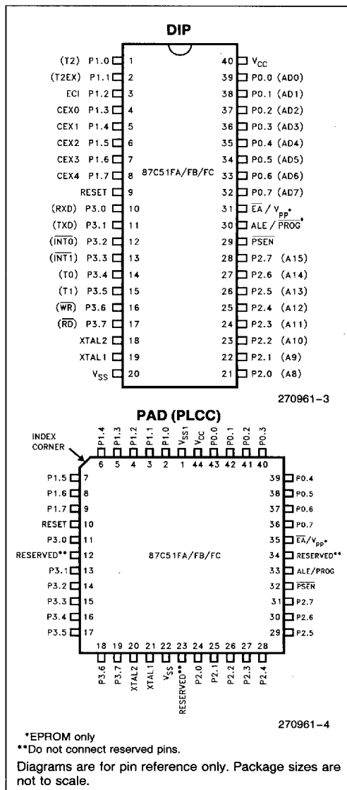
Figure 3. Pin Connections (Top View)
